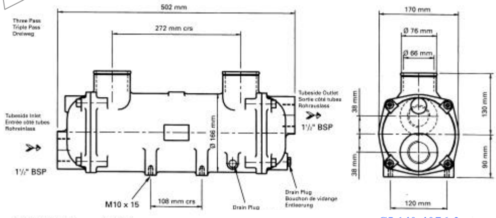
GL140-4076-2 suitable for engine up to 240kw (322HP)
