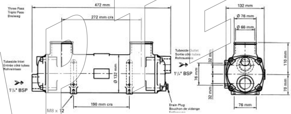
FG100-4075-2 suitable for engine up to 190kw (255HP)
